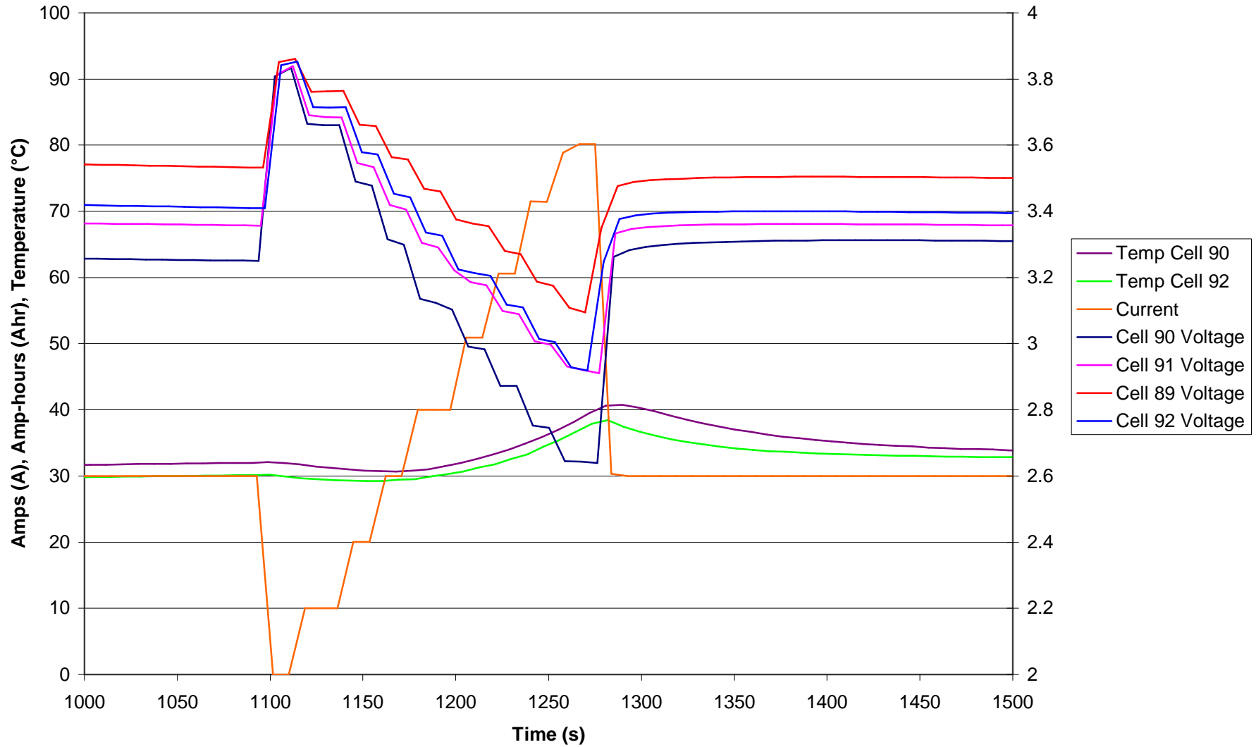
Discharge Cycle 6-17-03 w/ Fans blowing on cells for cooling expansion of resistance check area
