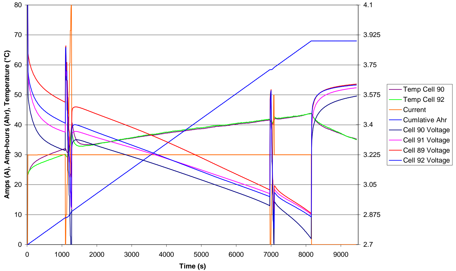
Discharge Cycle 6-17-03 w/ Fans blowing on cells for cooling
