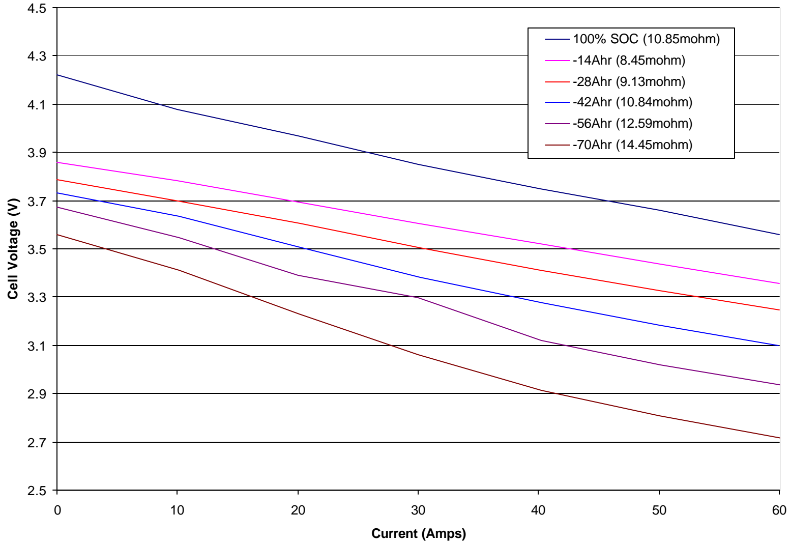
Li Ion Cell #89 Cell Voltage vs Load at various SOC (value in paranthesis is the equivalent series resistance)
