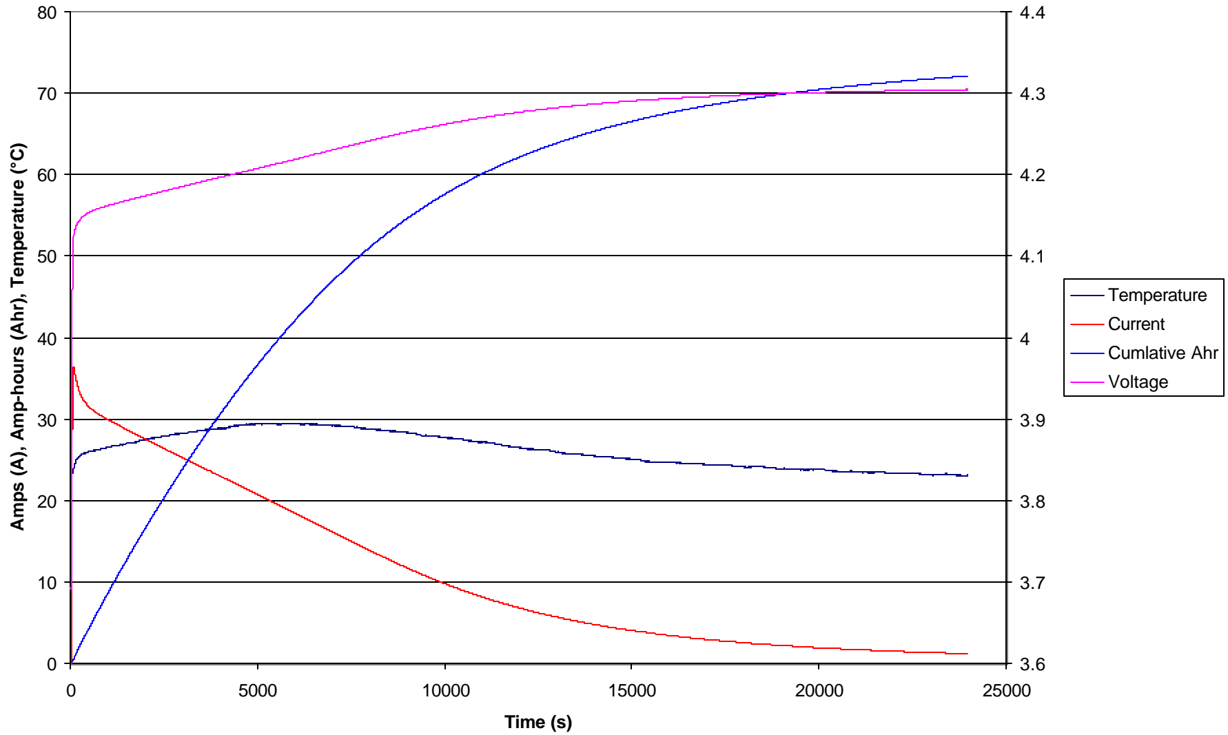
Charge Cycle #4 CV 4.3V with Series Resistance 5.8mohm
