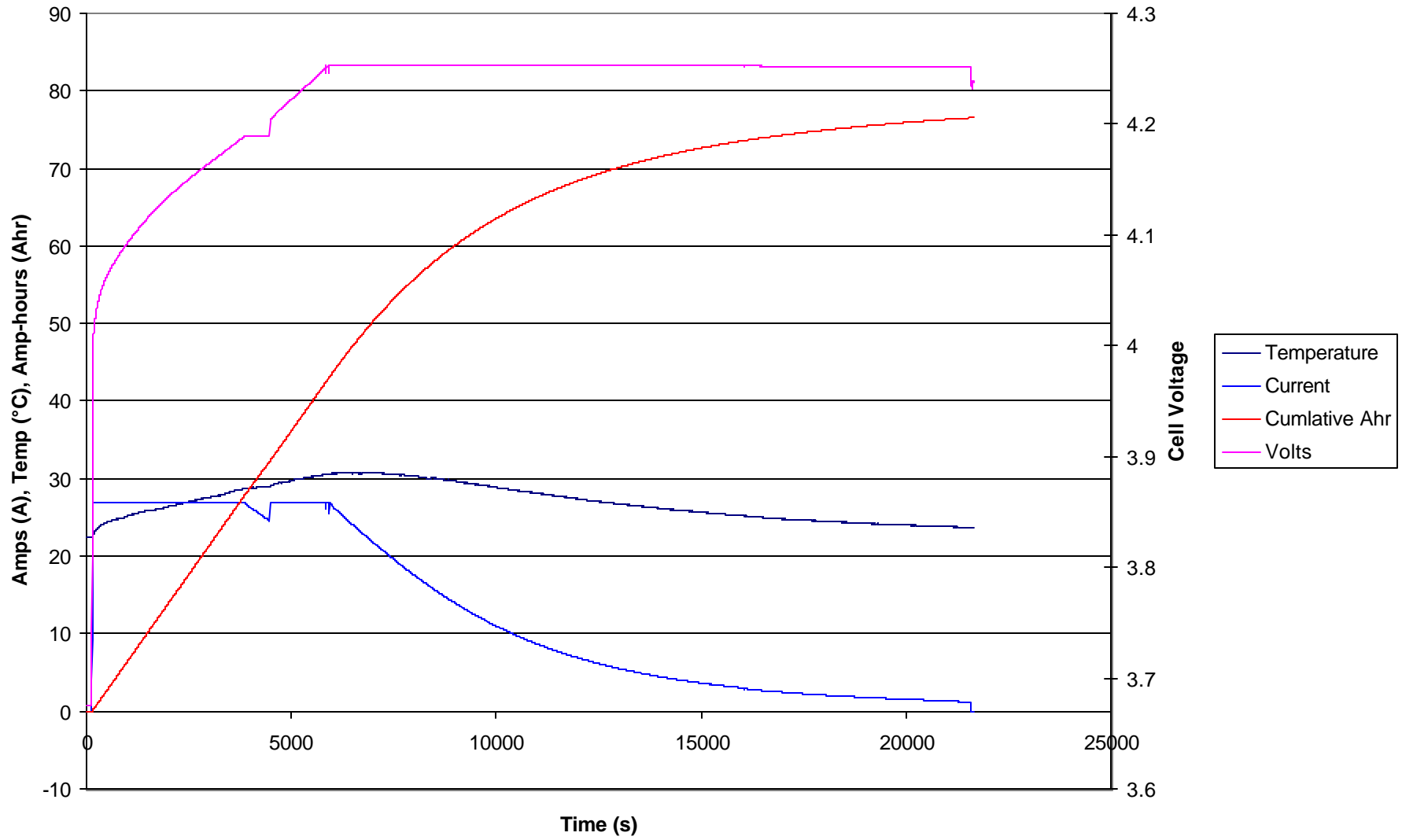
Cell #89 1st Charge Cycle 5-27-03
